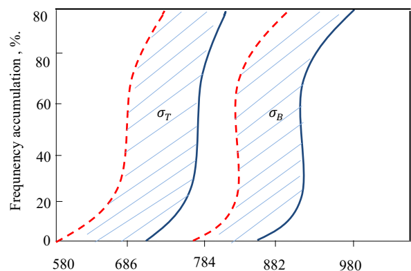
Figure 3. Cumulative curves of changes in strength properties depending on the strength coefficient and tempering temperature (V.Ya. Yankovsky, G.P. Prozorov, T.V. Soboleva): a) at a tempering temperature of 540-570 °C; b) 600-630 °C; 1) strength coefficient <0.67; 2) >0.67
