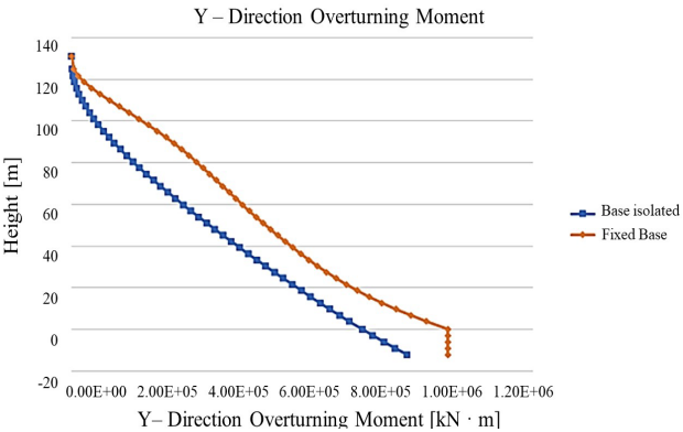
Figure 15. Overturning moment
