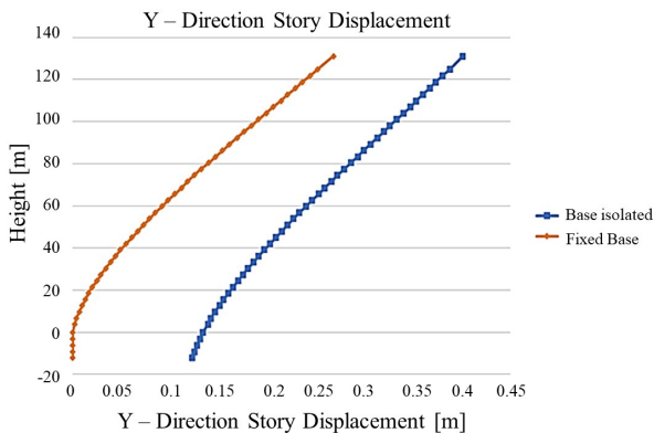
Figure 9. Story displacement
