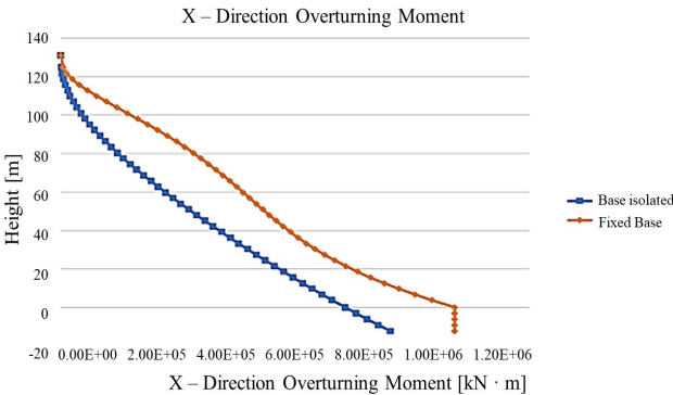
Figure 14. Overturning moment
