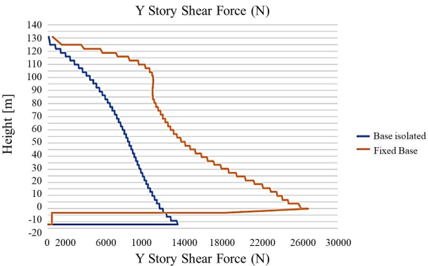
Figure 17. Story shear forces
