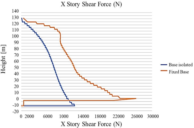
Figure 16. Story Shear forces
