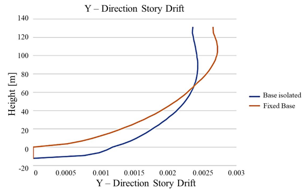
Figure 11. Story drift ratio
