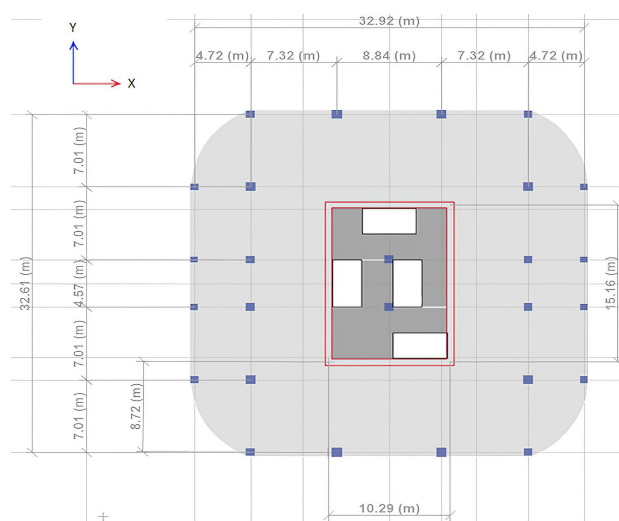
Figure 4. Typical floor plan [1, 2]
