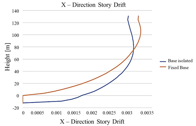
Figure 10. Story drift ratio
