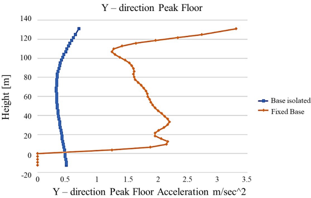
Figure 13. Floor acceleration
