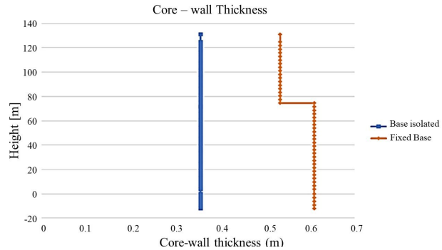
Figure 18. Reduction in core-wall section
